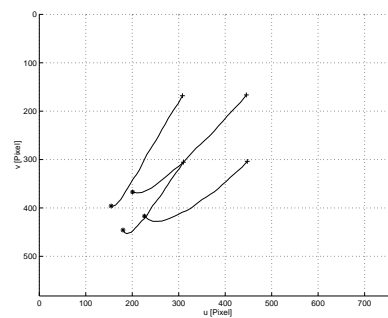
(b) Trust-Region-Regler, \alpha = 0.1 mm (27 Schritte)
