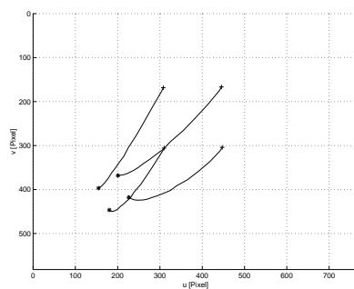
(c) Trust-Region-Regler, d_{soll} = 0.04 mm (16 Schritte)
